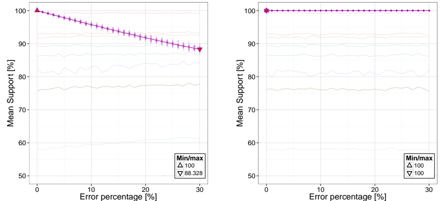
(a) The trend of the support of AtMostOne(a) , w.r.t. the percentage of spurious a’s inserted along the log (b) The trend of the support of AtMostOne(a) , w.r.t. the percentage of deleted a’s along the log
