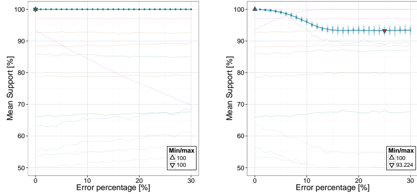
(a) The trend of the support of Participation(a) , w.r.t. the percentage of spurious a's inserted along the log (b) The trend of the support of Participation(a) , w.r.t. the percentage of deleted a's along the log
