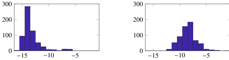
Figure 7: Histogram of \log_{10} of the backward error for a system as described in Subsection 6.7 of degree 25 using the Chebyshev basis (left) and the monomial basis (right).
