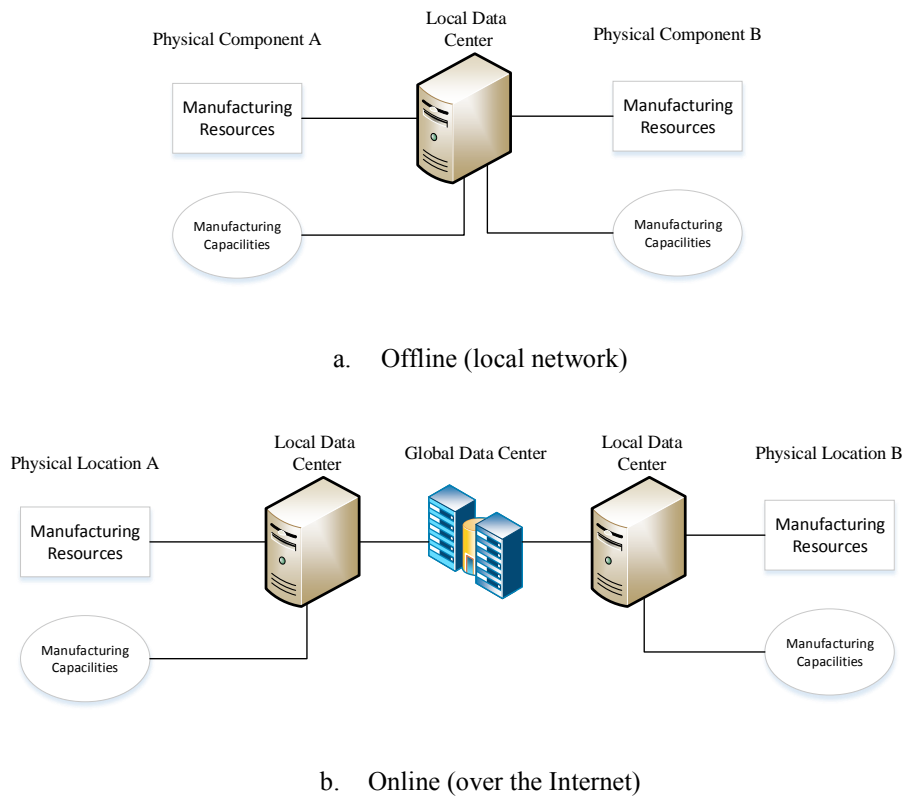
Fig. 1. CMS network
