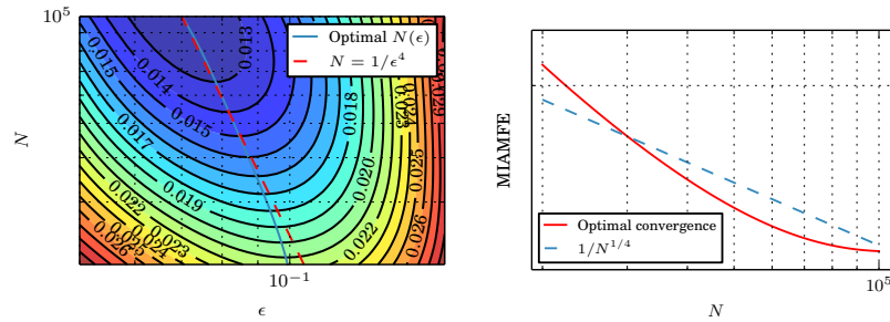
Fig. 1.6: L^1 error as a function of \epsilon and N (left). Optimal rate of convergence for the L^1 error (right)
