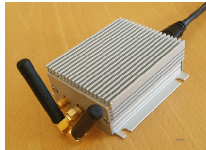
Figure 2. We built our own robust enclosure for the USRP boards and antennas.
