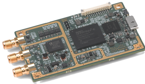
Figure 1. The Ettus Research B200mini USRP board, size 83.3 x 50.8 mm [11].
