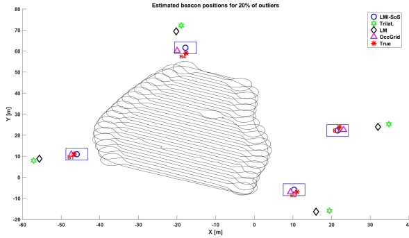
Fig. 11. Estimated beacon positions with 20% of outliers
