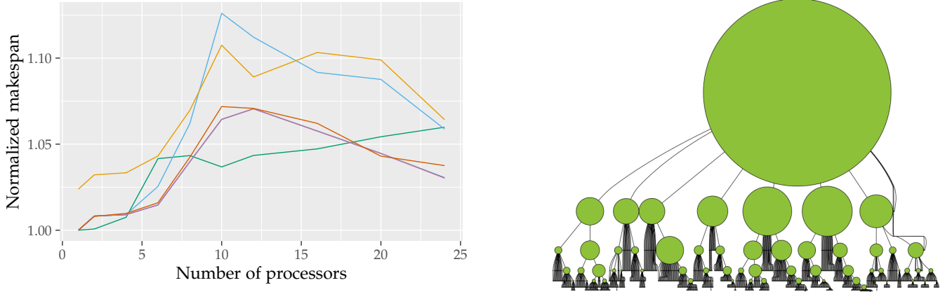
Figure 7: Performance of the heuristics and visual representation of the tree lp-nug30-colamd, where the area of a node is proportional to its sequential execution time.
