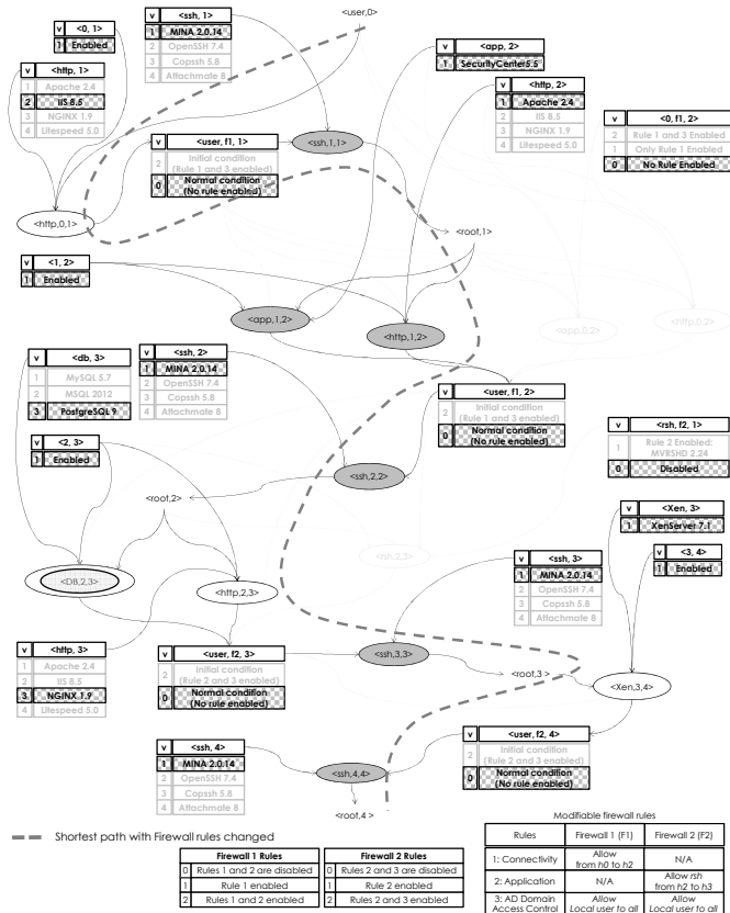
Fig. 4. Test case B: Effect of having an unpatchable vulnerability in the network.
