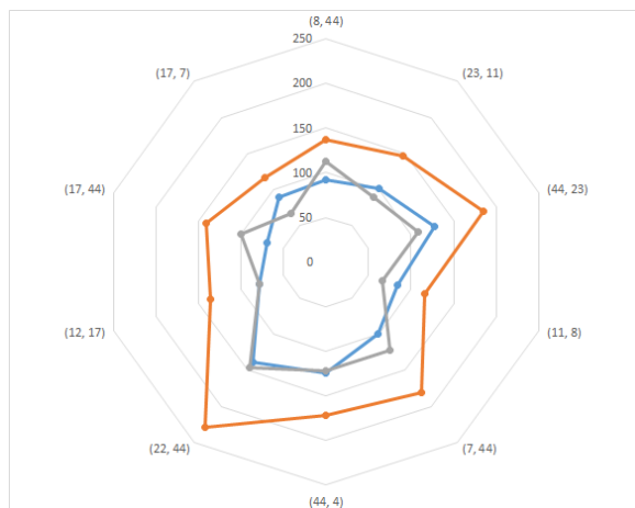
Fig. 2. Comparing the digraph model of three users.
