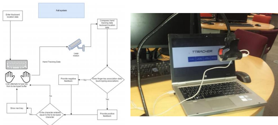
Fig. 1. (left) the prototype architecture (right) the physical setup
