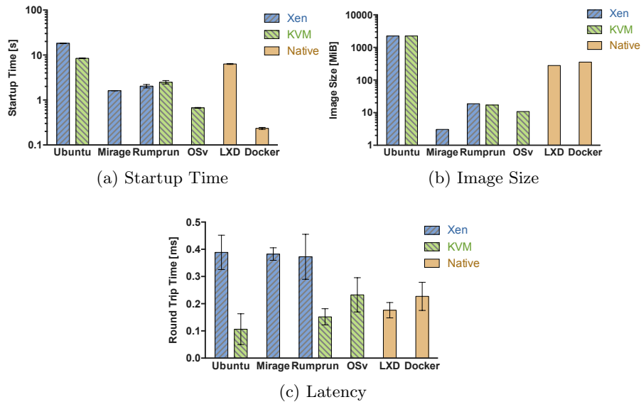
Fig. 3. A logarithmic scale is used to accommodate a wide range of values. (a) Startup time in seconds as measured using the procedure documented in [25]. (b) Image size in MiB as reported by the du utility. (c) Round-trip time in milliseconds as measured from a dedicated host.
