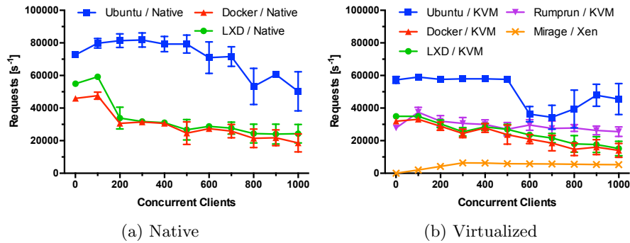
Fig. 4. Throughput of Nginx (1.8.0) was evaluated on native hardware (a) and in virtualized environments (b). For MirageOS, the conduit server was used. Throughput was measured using weighttp and the modified abc wrapper utility.
