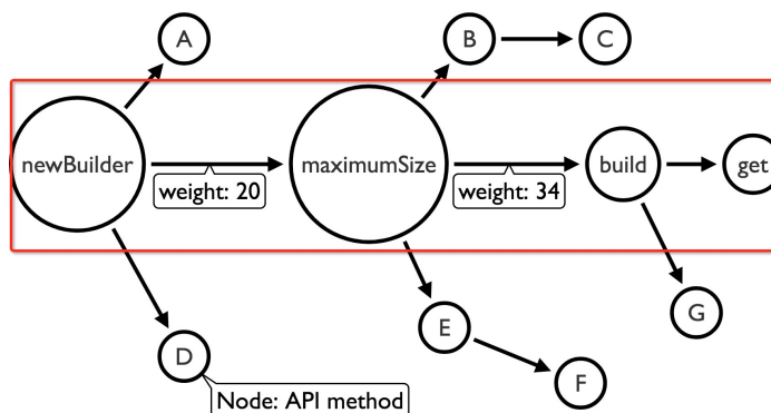
Fig. 4. Method Sequence Call Graph Demo
