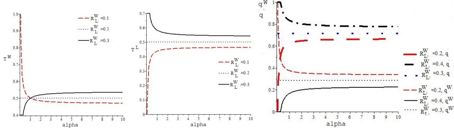
Fig. 1. Wi-Fi throughput (left), LTE-U throughput (middle) and fraction of time for only Wi-Fi network's access and joint access the channels (right) as functions on fairness coefficient.
