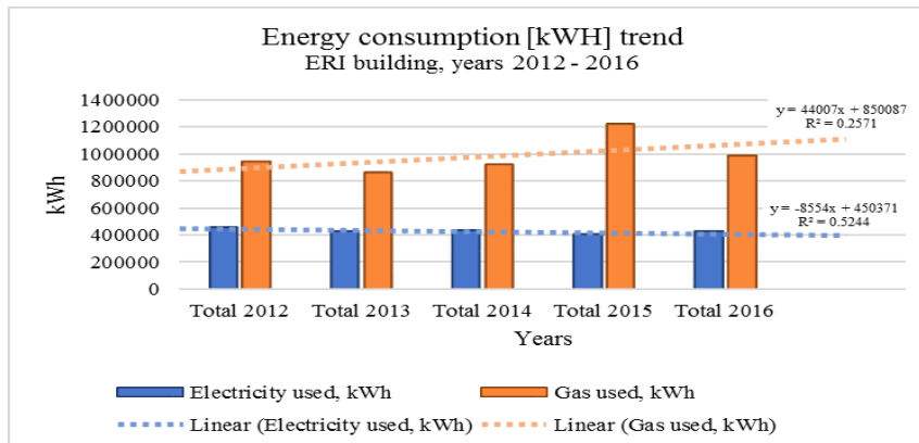
Fig. 5. The ERI energy consumption trend for the last five years.
