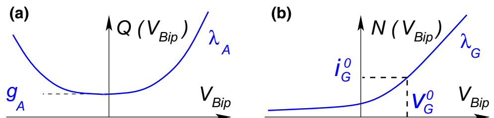
Fig. 3 Transmission functions of the model. (a): Activation function Q(V_{\text{Bip}}) for shunt conductances g_A in bipolar cells. (b): Synaptic transmission N(V_{\text{Bip}}) from bipolar to ganglion cells
