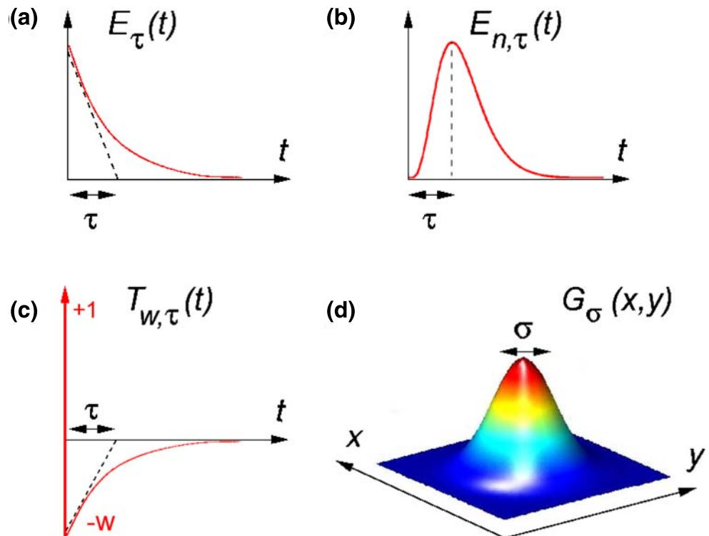
Fig. 2 Linear kernels used in the model. (a): Exponential kernel E_{\tau}(t) (temporal, low-pass). (b): Gamma (exponential cascade) kernel E_{n,\tau}(t) (temporal, low-pass). (c): Partially high-pass kernel T_{w,\tau}(t) (temporal, high-pass). (d): Gaussian kernel (spatial, low-pass)
