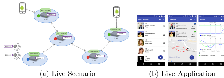
Figure 9: Tracking runners
