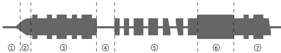
Fig. 4. Simplified ATA5577C [1] timing diagram during read and write operations. When the tag enters the RF field (1), the power-on reset circuit remains active until the internal capacitor is charged and an adequate voltage threshold is reached (2). After a default initialization delay (usually about 3 ms after entering the RF field), the tag enters regular read mode. In the normal mode, data is encoded according to the configuration registers of ATA5577C and transmitted from the first stored data block (3). Most configurations use Manchester ASK modulation. To switch the tag from reading to writing mode, the card reader must interrupt the RF field for a short time (4), typically for 64 – 400 μs. After the successful mode switch, the tag enables (by default) the damping. A sequence of operational code, lock bits, address and data block must follow (5). Data bits are encoded by an on-off modulation with write gaps of 64 - 160 μs. The programming sequence is terminated with the programming delay of 5.6 ms. This delay is necessary for correct programming. After programming, the tag returns to block-read mode and transmits last written block (7).
