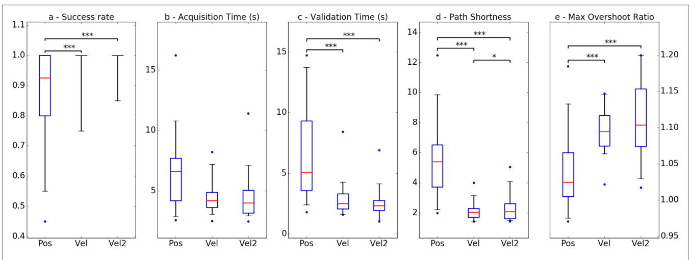
FIGURE 5 | Evolution of performance between modes regarding the five quantitative metrics. Boxplots display the values' distribution as follows: the box extends from lower to upper quartile values with a red line at the median, and the whiskers extend from the box to 5th and 95th percentile values. Flier points are considered outliers. Pairs of modes presenting significant differences are indicated with stars: * p < 0.05 , ** p < 0.01 , *** p < 0.001 . (A) Success rate, (B) acquisition time (s), (C) validation time, (D) path shortness, and (E) max overshoot ratio.
