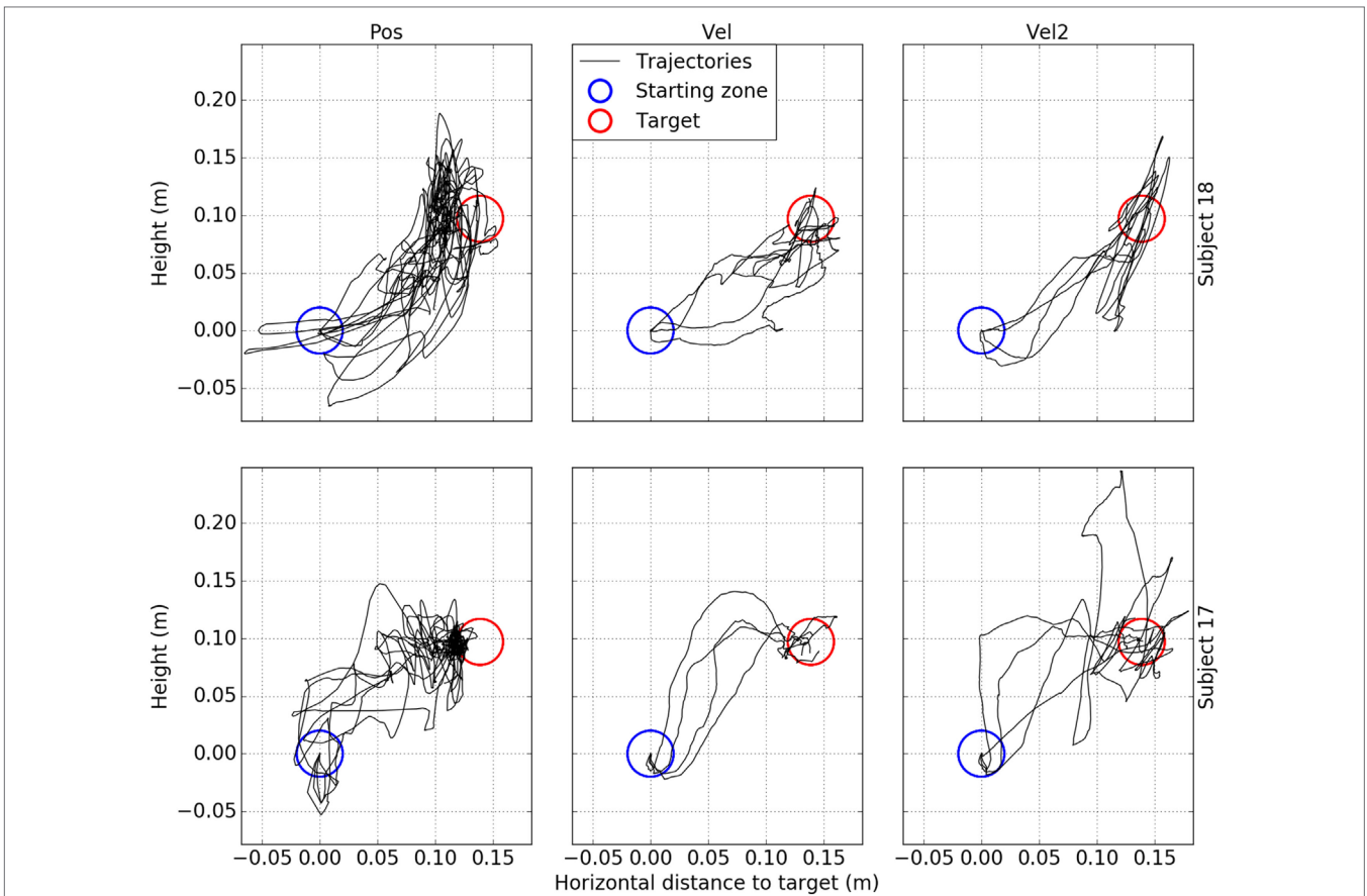
FIGURE 4 | Examples of endpoint trajectories generated with each control mode. The data are taken from twenty-four trials performed by subjects #17 (bottom row) and #18 (top row). Each chart illustrates four trials performed by the same subject with the same mode and aiming at the same target (target B). Each column corresponds to one of the three control modes. The trajectories (in black), target (in red) and starting zone (in blue) are projected onto the vertical plane joining the starting point and the target center.
