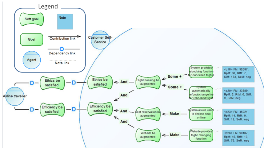
Fig. 6. Generated i* SRM model
