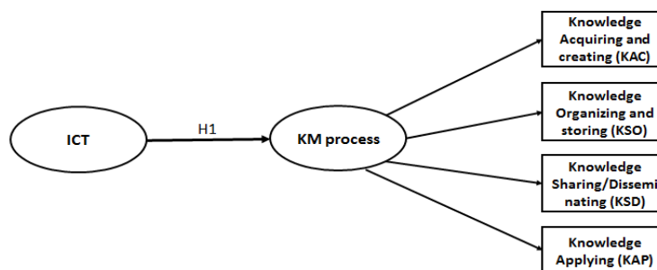
Fig. 1: Research framework
