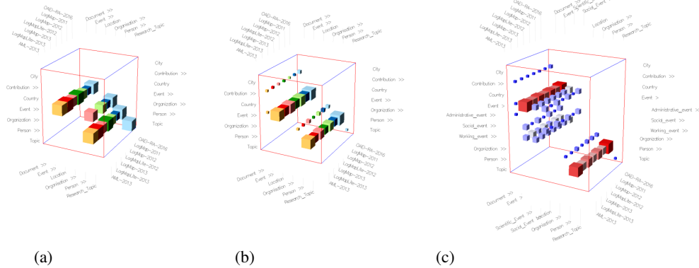
Fig. 3: Alignment Cubes for visualizing ontology alignments. Rows and columns of the cube represent ontology concepts, individual cells inside the cube represent mapping relationships. Each alignment, corresponding to a slice in the third dimension, is assigned a different color. (a) Default view in similarity values mode. (b) Initial view in mappings mode. (c) Mappings mode with cell weight color encoding after expanding the Events concepts in both ontologies.
