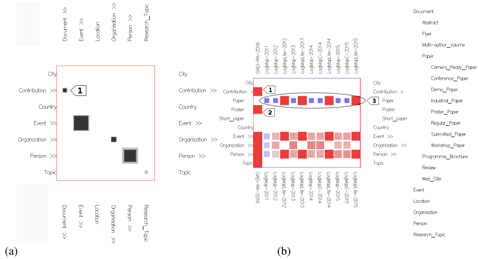
Fig. 7: Aggregated projections: (a) alignment topology and (b) concept networks.
