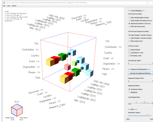
Fig. 2: Alignment Cube UI. Widgets (sliders, button groups, etc.) mentioned in the text are referred to directly using their name. The cubelet (bottom left corner) is used to switch between views by clicking or dragging the mouse on its faces.
