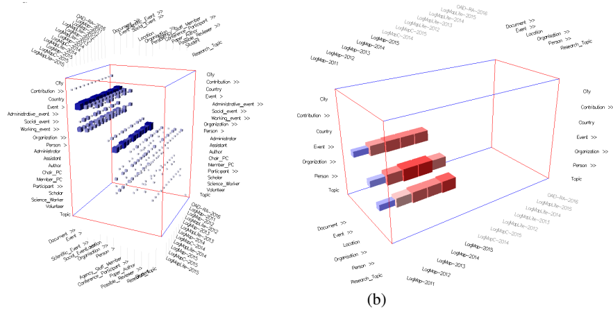
Fig. 5: Views of Alignment Cubes: (a) after expanding concepts and (b) after filtering out several alignments.
