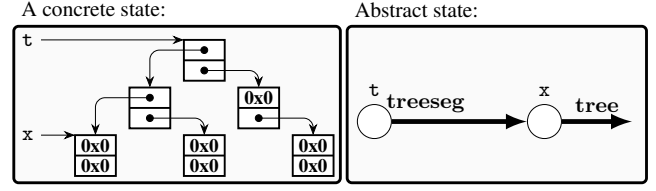
Figure 3. Abstract states.
