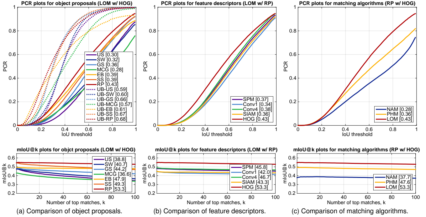
Fig. 5. PF-PASCAL benchmark evaluation on region matching precision (top, PCR plots) and match retrieval accuracy (bottom, mIoU@ k plots): (a) Evaluation for LOM with HOG [46], (b) evaluation for LOM with RP [24], and (c) evaluation for RP with HOG [46]. The AuC is shown in the legend. (Best viewed in color.)
