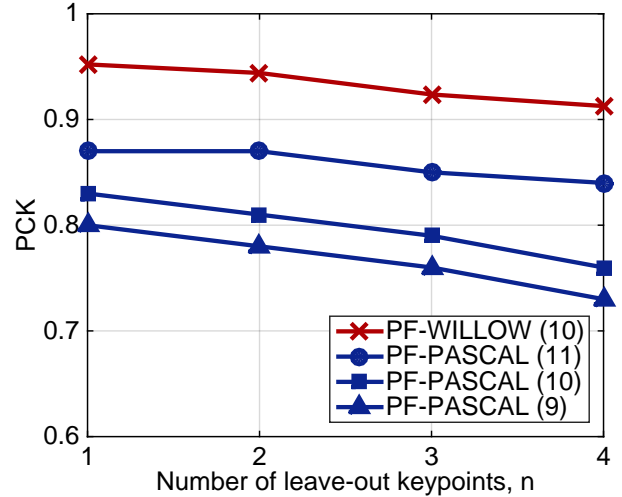
Fig. 9. Verification of ground-truth data using a leave- n -out validation. This shows the average PCK of 10 trials over all object classes. For this experiment, we leave out n randomly selected keypoints per each pair, and then measure PCK scores between the estimated correspondences (using TPS warps) of the leave out keypoints and their ground-truth annotations. (Best viewed in color.)
