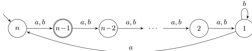
Fig. 4. The binary witness for reversal meeting the bound 2n + 1 .
