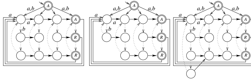
Fig. 1. The witnesses for SVFA-to-DFA conversion; n = 13, 12, and 14 .
