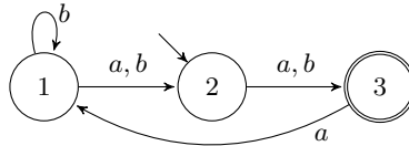
Fig. 3. An NFA for the language L in Example 6.
