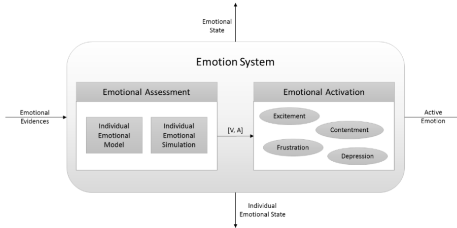
Fig. 3. Emotion System
