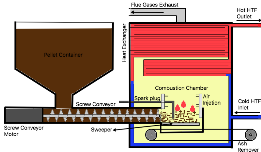
Fig. 2. Operating principle of the pellets boiler.
