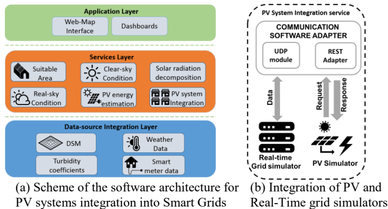
Fig.1. PVInGRID infrastructure
