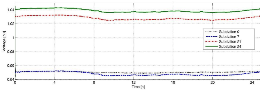
Fig.3. Voltage profile for substations 7-9-22-24
