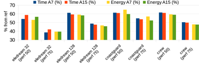
Fig. 2. Run time and energy consumption for the x264-encoder
