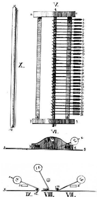
Fig. 5 Rectilinear Homeoscope with movable parts
