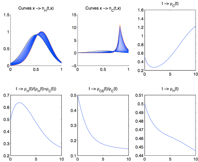
Figure 1. Simulation with u_1(t) = Cst = 3.5 and u_2(t) = Cst = 2 , in time T = 10 . Here \rho_{CS}(t) = \int_0^1 (1-x)n_C(t,x) dx is a measure of the number of sensitive cells in the cancer cell population.
