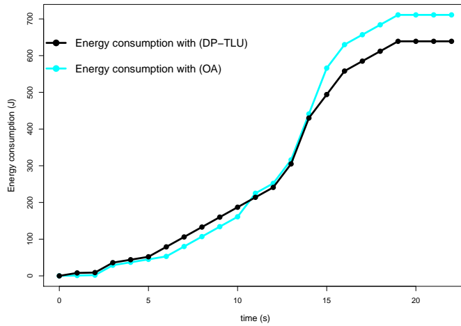
Figure 6: Comparison of the energy consumption between (OA) and (TLU DP ) solutions, with fixed deadlines d_n = 3 , size c_n \in \{0, 2, 4\} with respective probabilities (0.2, 0.6, 0.2), and processor speeds in \{0, 1, 2, 3, 4\} .
