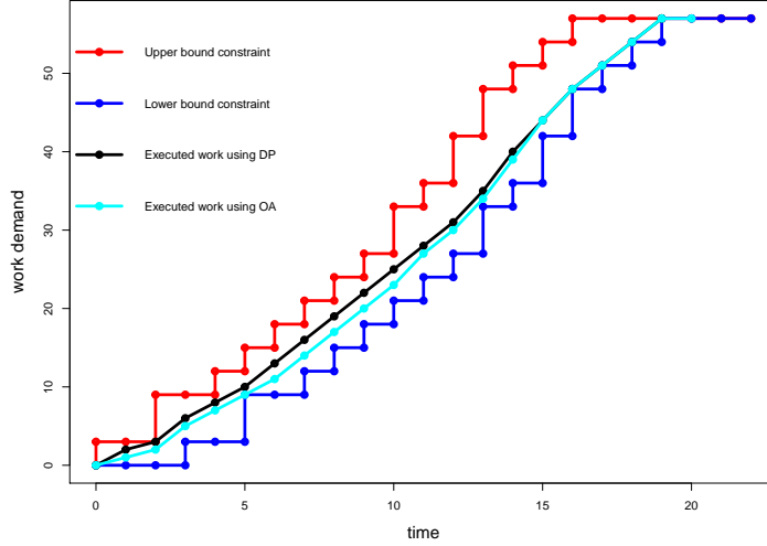
Figure 5: Comparison of the executed work between (OA) and (TLU DP ) solutions, with fixed deadlines d_n = 3 , size c_n \in \{0, 2, 4\} with respective probabilities (0.2, 0.6, 0.2), and processor speeds in \{0, 1, 2, 3, 4\} .
