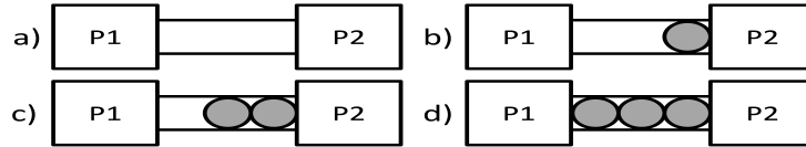
Fig. 3. All combinations of two processes with a buffer inventory capacity of three parts
