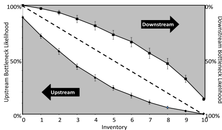
Fig. 7. Bottleneck location for a system with identical exponential distributed cycle times
