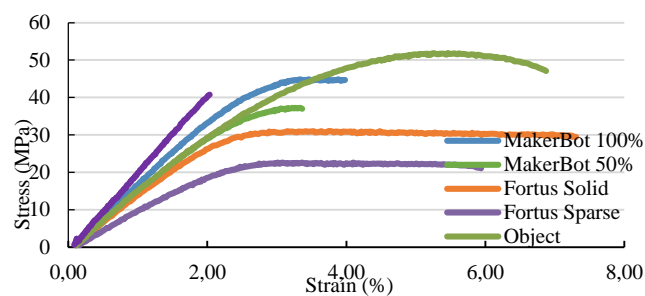
Fig. 6. Stress-strain curve comparison
