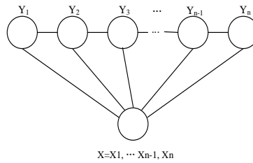
Fig.1. CRFs Model
