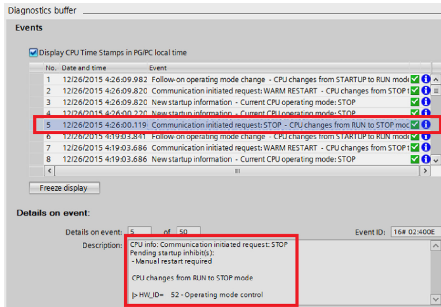
Figure 8. Event log generated by sending a STOP command.
