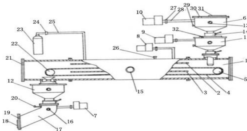
Figure1. Experimental configuration for low-temperature plasma treatment
