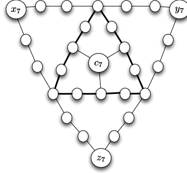
Fig. 2: Example of T_\gamma . Edges are bold only to better distinguish the different “levels”.
