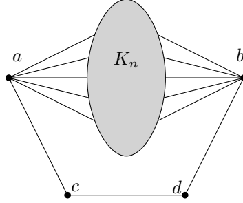
Fig. 1: A family of graphs with lattice of convex subgraphs being arbitrary far from ranked.
