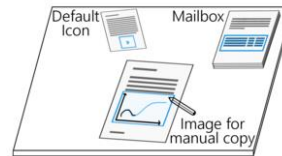
Fig. 8. Semantic-Pinch use
