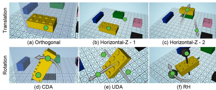
Fig. 1. Proposed 3D object manipulation techniques for unconstrained viewpoints. The green circles represent user touches and the gray arrows the movement of these touches.
