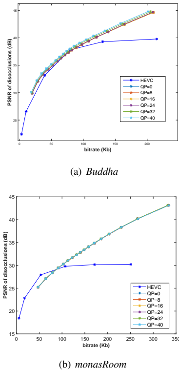
Fig. 4. Results of coding the disoccluded pixels using a Graph-based approach(QF from 10 to 90) vs HEVC (QP 0 to 40) for Buddha and monasRoom
