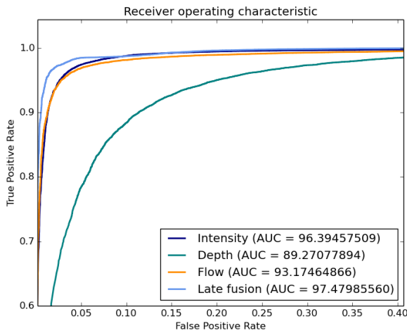
(c) Incremental cross-modality training using best modality specific setting
