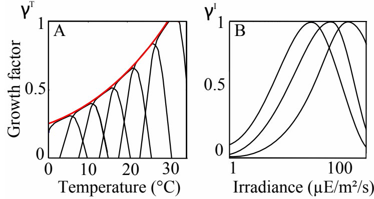
Fig. 8 A, Eppley curve normalized at 30°C. B, photosynthesis as represented in eq. 38. The figure is redrawn after Follows et al (2007).
