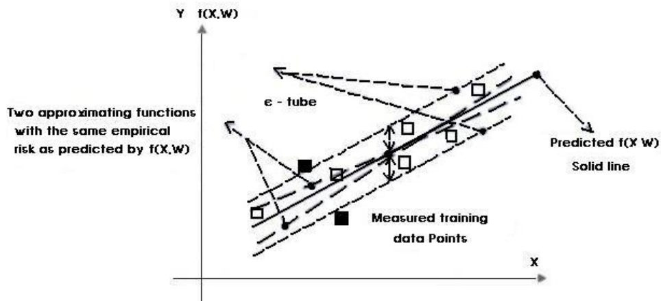
Figure 1. \varepsilon -SVR for Regression
