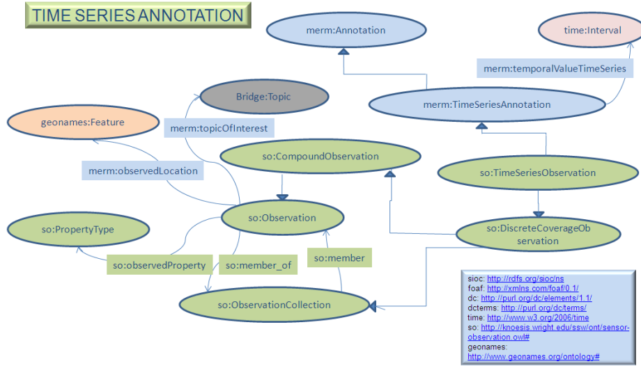
Fig. 4. TimeSeriesAnnotation model
