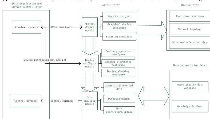
Fig. 3. Software architecture
