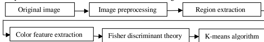
Fig. 6. Flow chart of maize seed feature analysis and identification
