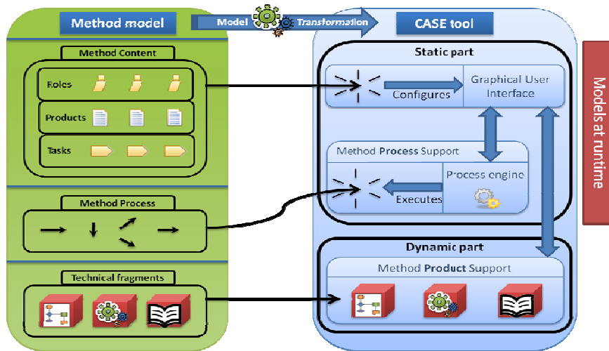
Fig. 10. Transformation mappings
