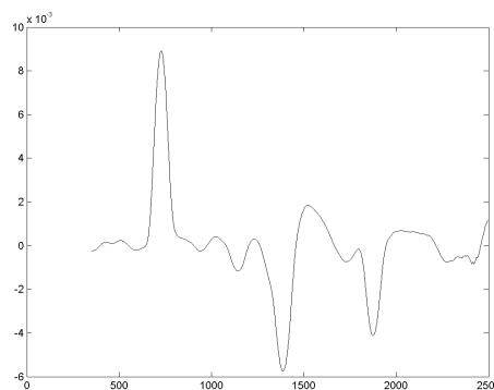
Figure 6. Kernel smoothing after the first derivative
