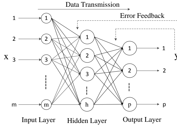
Fig.2. The BP neural network topology
