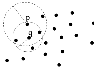
Fig. 2. 4 - dist values for example core ( q ) and border point ( p )
