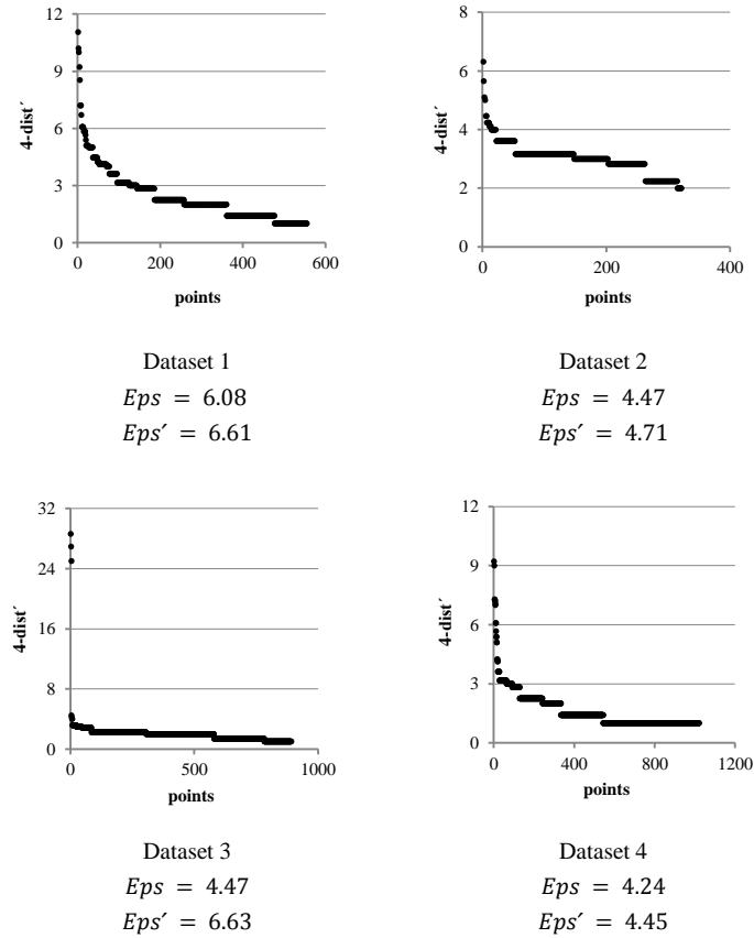
Fig. 5. Sorted 4 - dist' graphs for sample datasets 3
